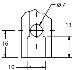
Mill Detail
