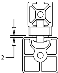
Clearance dimensions
