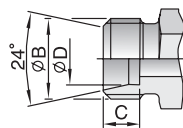
without O-ring
