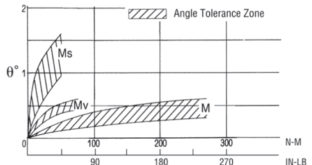
63 mm Bore
