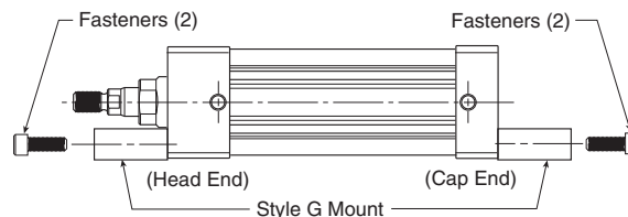
Fig. 4 - Side End Lug Mounting Kit - Style MS7
